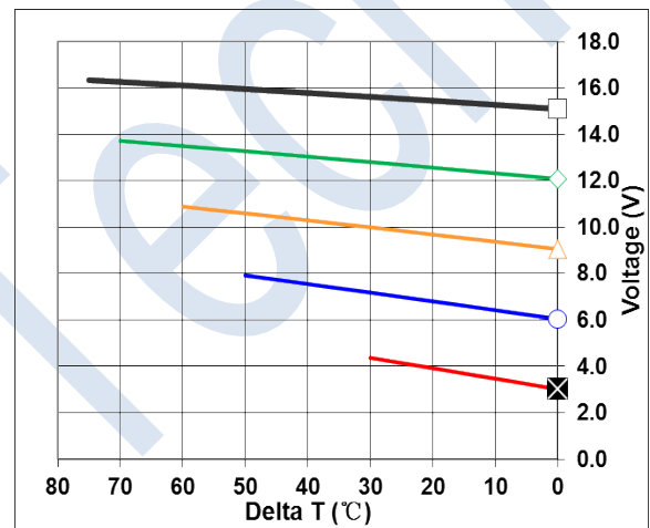
Performance Curves Th=50 °C
